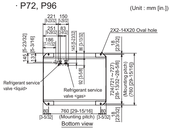
Installation base parallel to the unit's front panel
