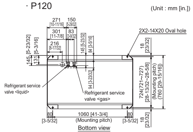
Installation base perpendicular to the unit's front panel
