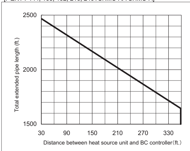
[PQRY-P144, 168, 192, 216, 240TSHMU-A/YSHMU-A]
