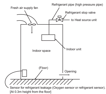
Fig.6-4. Fresh air supply and refrigerant shut-off upon sensor action
