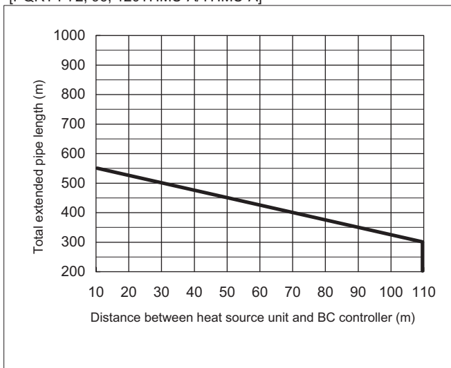
[PQRY-P72, 96, 120THMU-A/YHMU-A]
