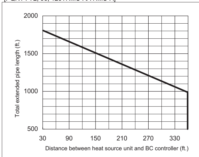
[PQRY-P72, 96, 120THMU-A/YHMU-A]
