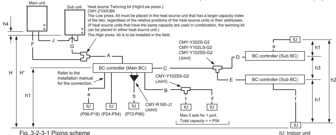
Fig. 3-2-3-1 Piping scheme
