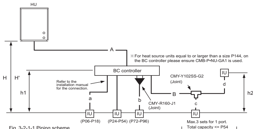
Fig. 3-2-1-1 Piping scheme
