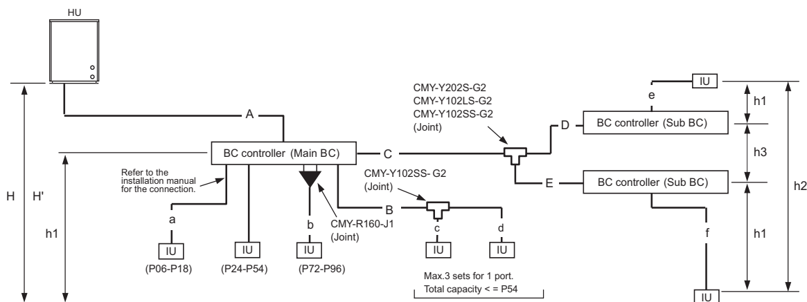
Fig. 3-2-2-1 Piping scheme
