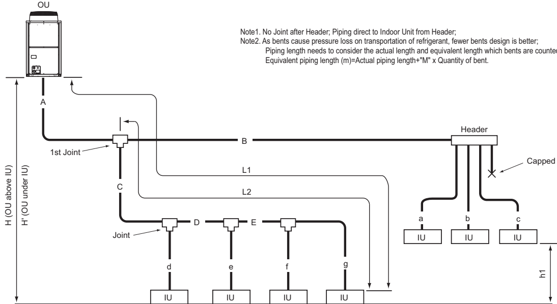
Fig. 3-2-1A Piping scheme
