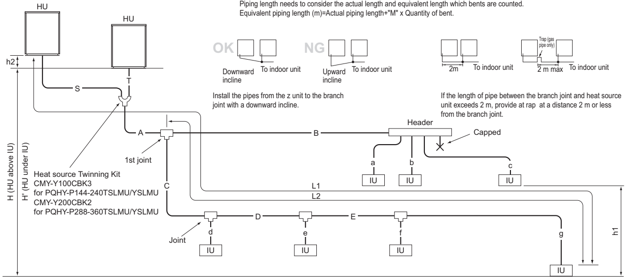
Fig. 12-2-1B Piping scheme
