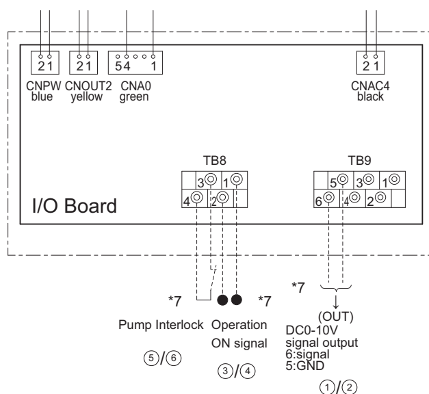
Figure d)-2 I/O board wiring diagram
