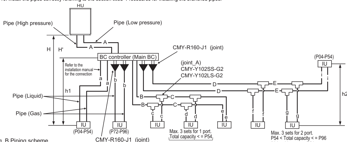
Fig. B Piping scheme
