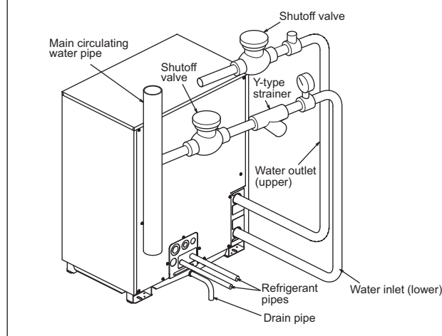
Installation example of heat source unit
