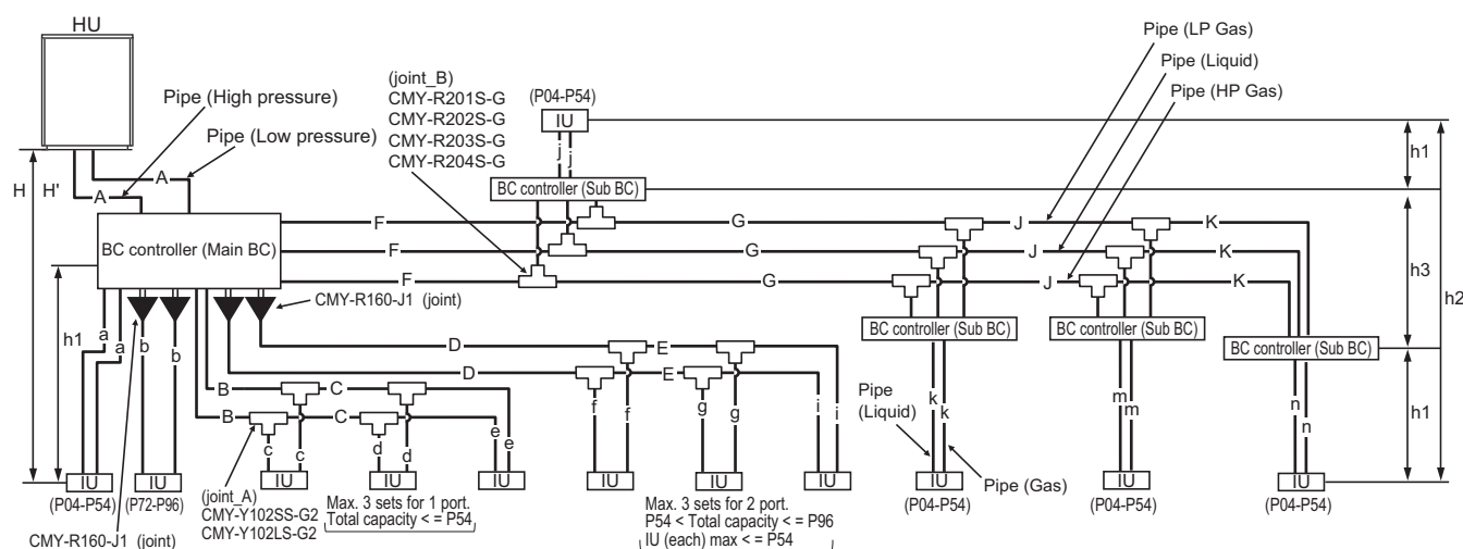
Fig. B Piping scheme
