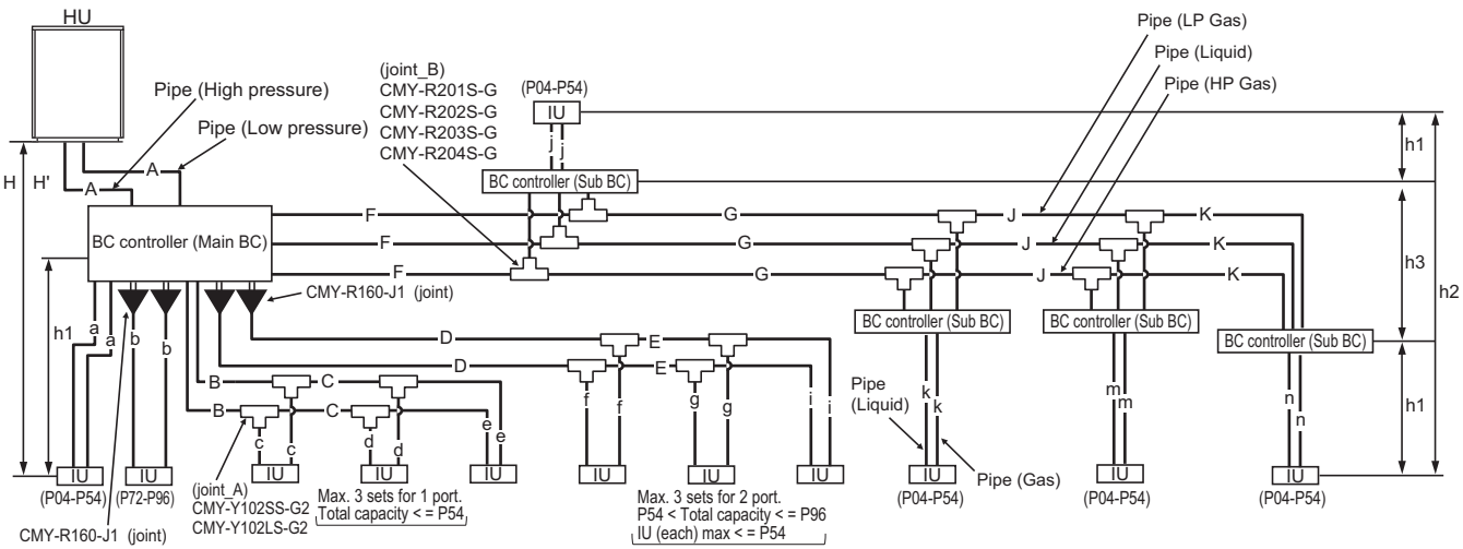
Fig. 12-2-2A Piping scheme
