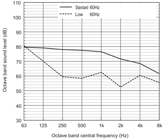
Sound level of PUHY-HP120T(Y)NU
