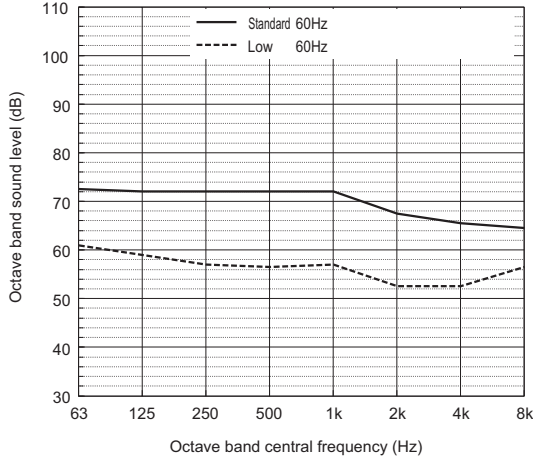
Sound level of PUHY-HP72T(Y)NU
