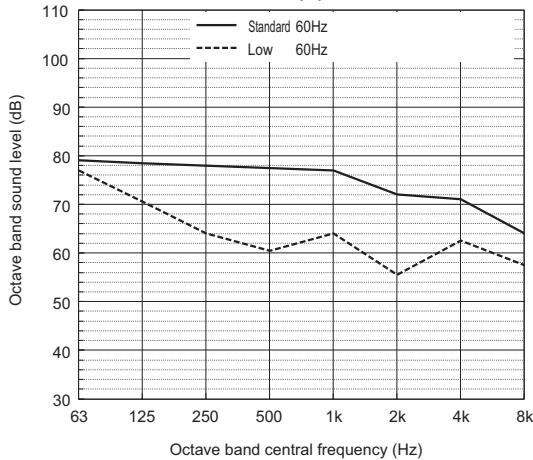
Sound level of PUHY-HP192T(Y)SNU
