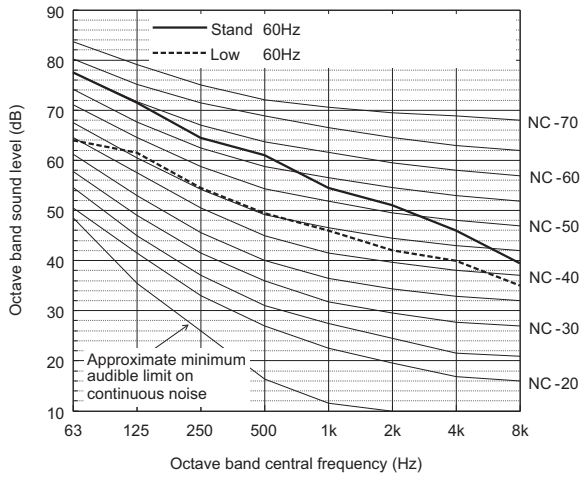
Sound level of PUHY-P240ZSKMU-A(-BS)
