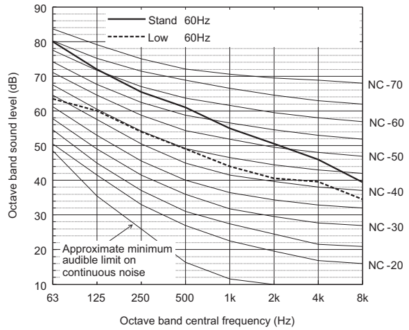
Sound level of PUHY-P264ZSKMU-A(-BS)
