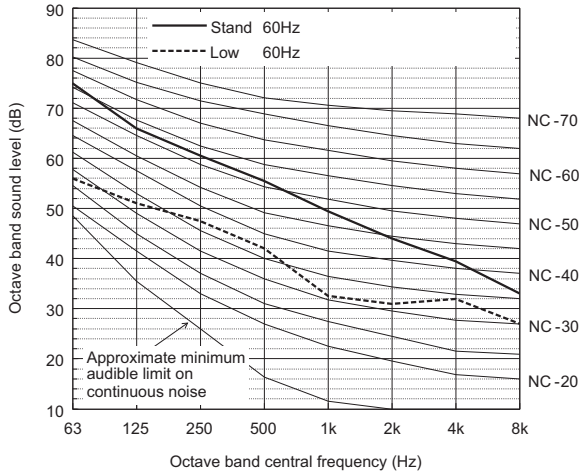
Sound level of PUHY-P72ZKMU-A(-BS)
