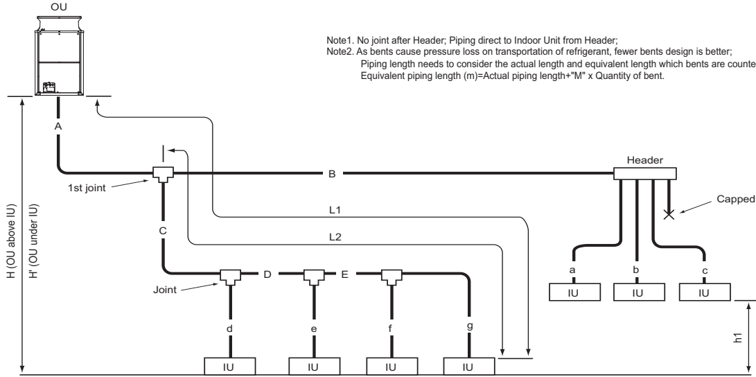
Fig. 3-2-1A Piping scheme
