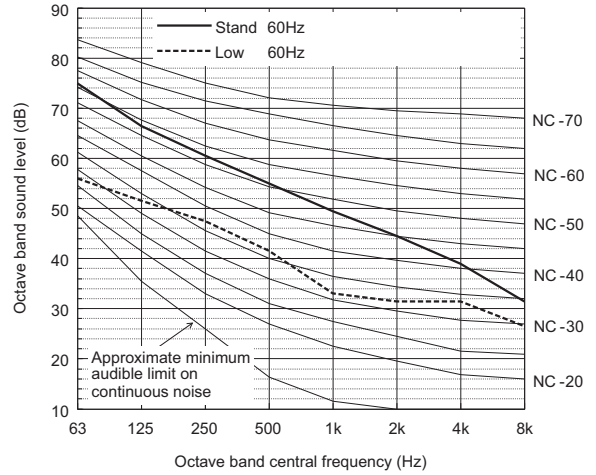
Sound level of PUHY-P96ZKMU-A(-BS)
