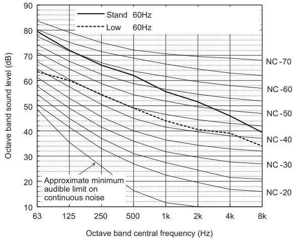
Sound level of PUHY-P288ZSKMU-A(-BS)
