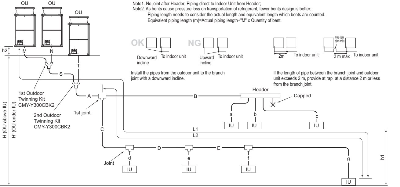
Fig. 3-2-1C Piping scheme
