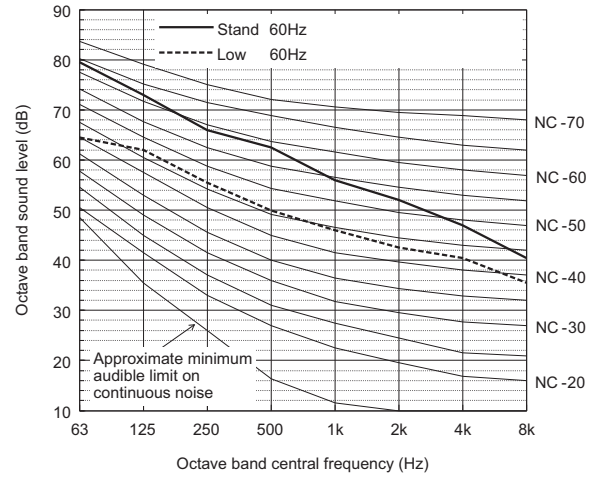
Sound level of PUHY-P312ZSKMU-A(-BS)
