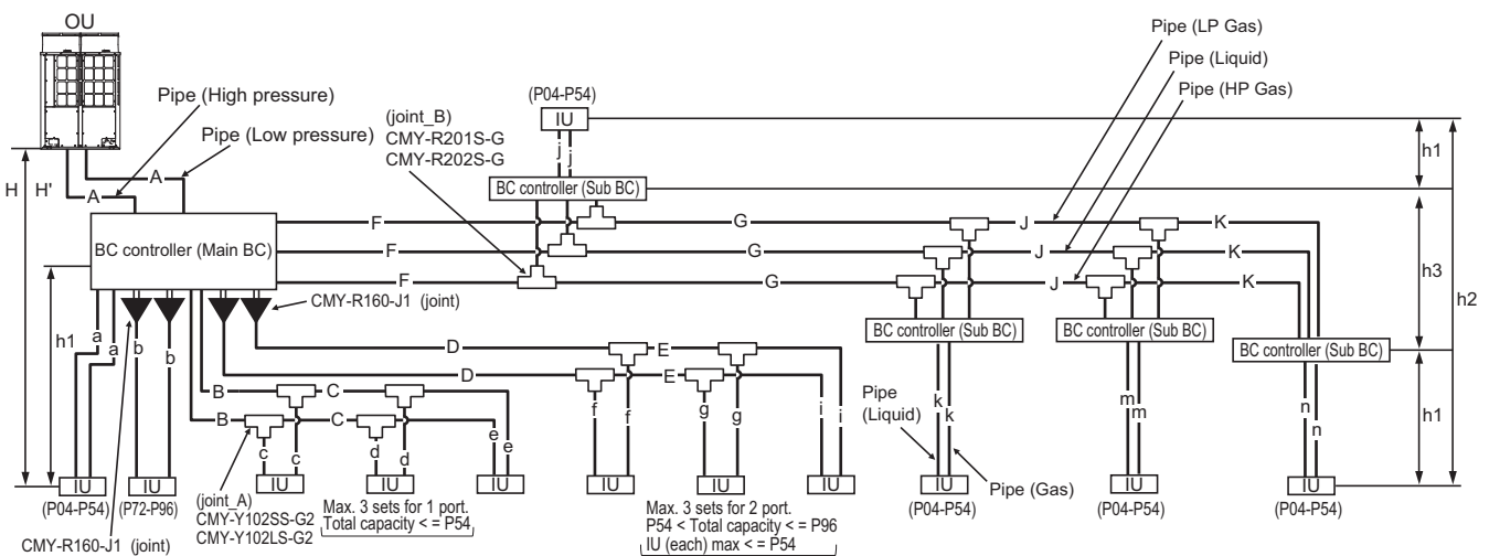
Fig. 12-2-2A Piping scheme
