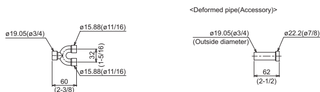
High-pressure twinning pipe
