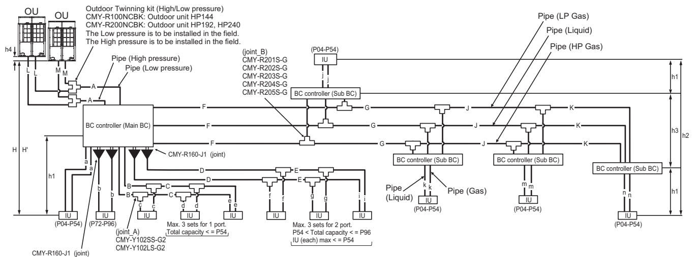
Fig. 12-2-3A Piping scheme
