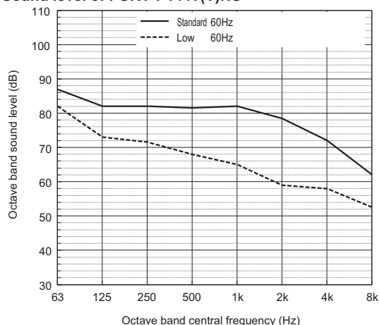
Sound level of PURY-P144T(Y)NU
