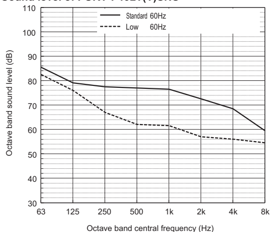
Sound level of PURY-P192T(Y)SNU
