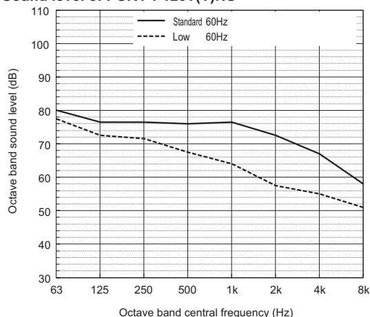
Sound level of PURY-P120T(Y)NU
