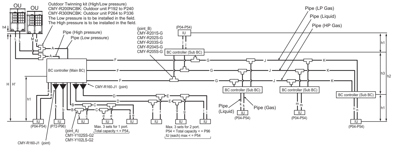
Fig. 12-2-3A Piping scheme
