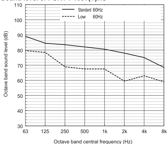
Sound level of PURY-P168T(Y)NU
