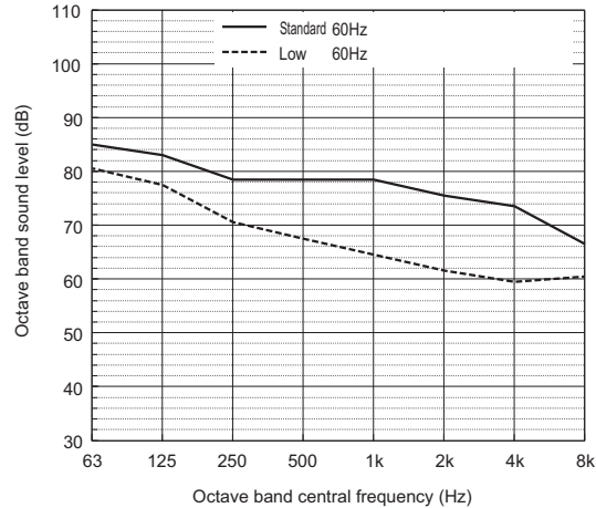
Sound level of PURY-P216T(Y)SNU
