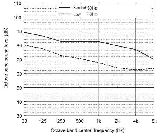
Sound level of PURY-P264T(Y)SNU
