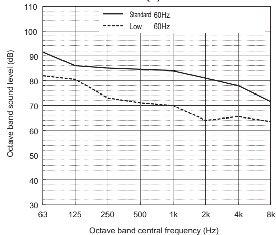
Sound level of PURY-P312T(Y)SNU
