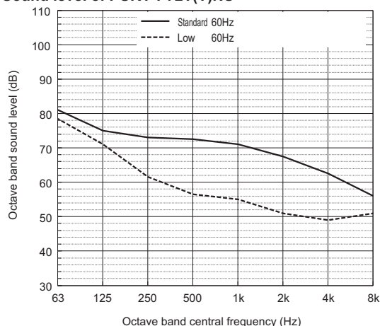
Sound level of PURY-P72T(Y)NU
