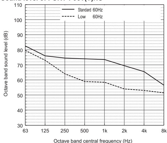
Sound level of PURY-P96T(Y)NU
