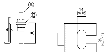
Hanging method
