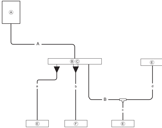
[PQRY-P72~P240TLMU-A1/YLMU-A1]
