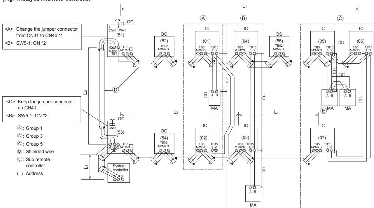
[Fig. 11.3.2] MA Remote Controller
