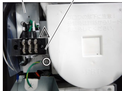
TB fix plate Terminal block
