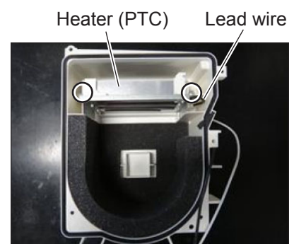
Blower (assy)
