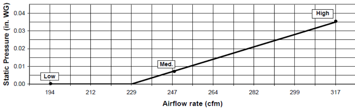
PEFY-P08NMSU-ER2 with Filter Box FBL1-1
