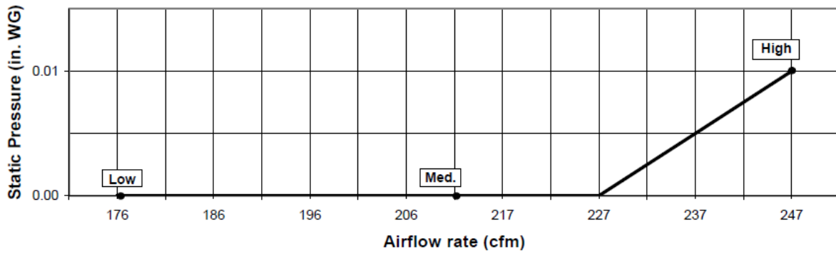
PEFY-P06NMSU-ER2 with Filter Box FBL1-1
