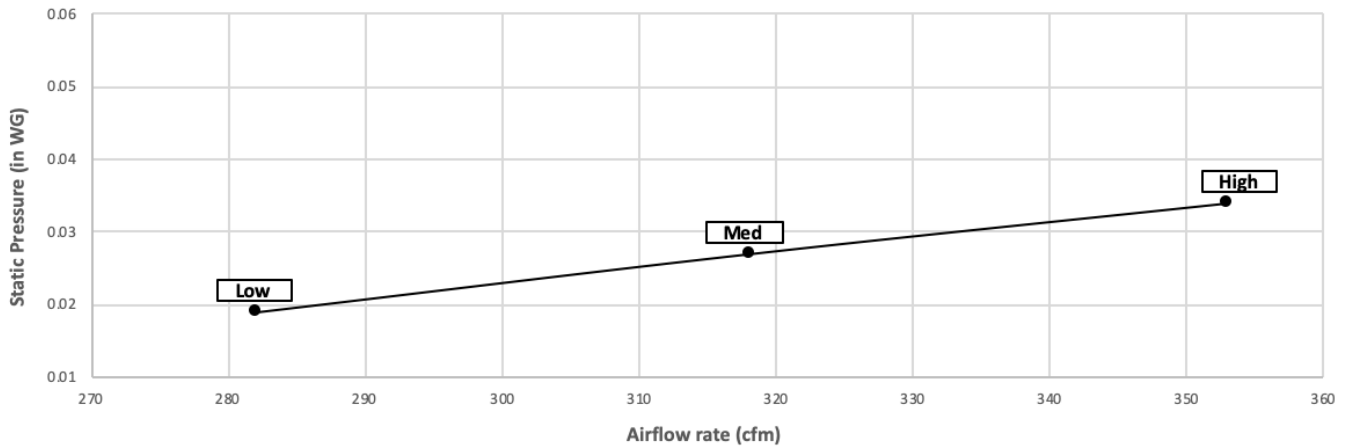
PEAD-A09AA8 with Filter Box FBM2-2-A
