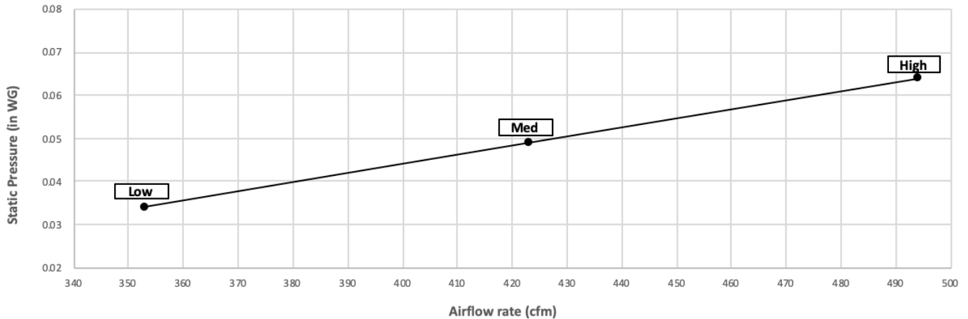
PEAD-A12AA8 with Filter Box FBM2-2-A
