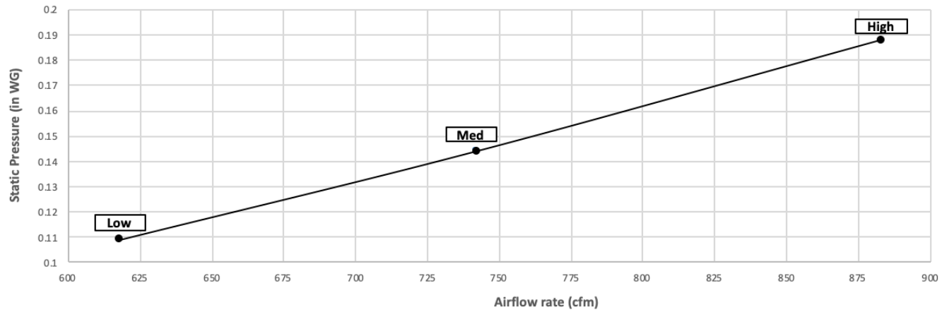
PEAD-A30AA8 with Filter Box FBM2-3-A
