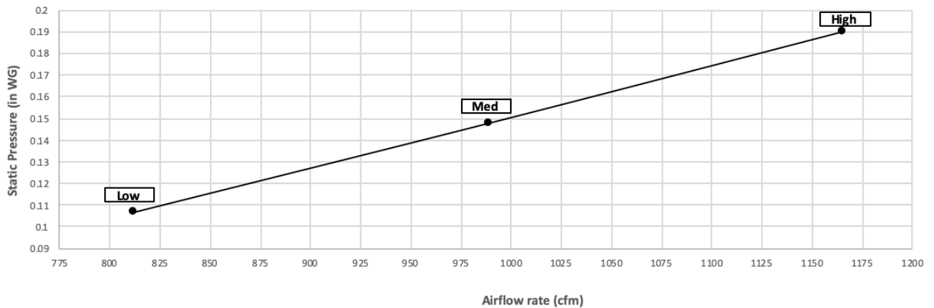
PEFY-P36NMAU-E4 - P30NMAU-E5 with Filter Box FBM2-4-A
