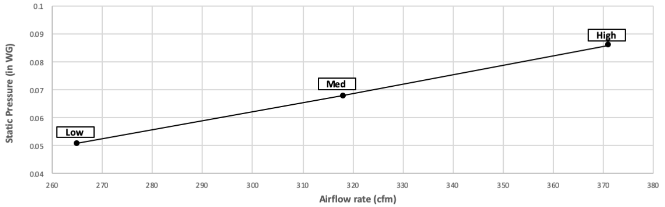
PEFY-P12NMAU-E4 with Filter Box FBM2-1-A
