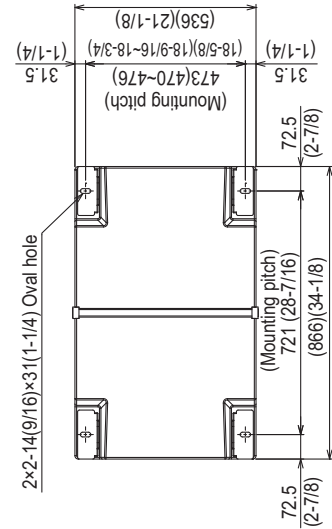
Bottom view
