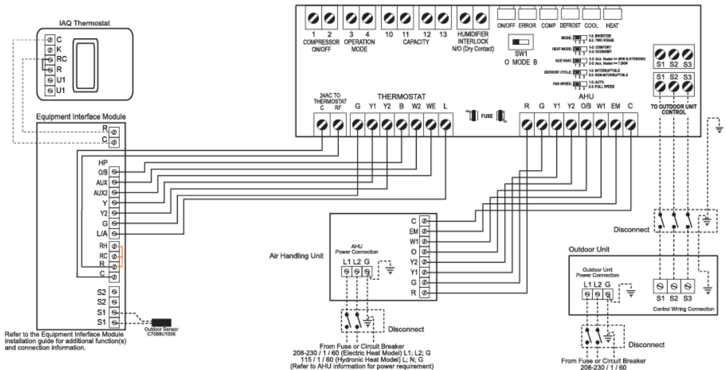
BVRMC1137S001-D4 System Wiring Diagram
