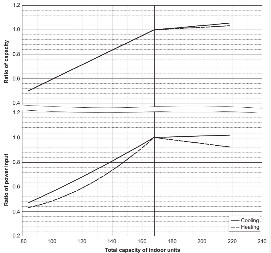
PQHY-P192T(S)LMU/Y(S)LMU-A
