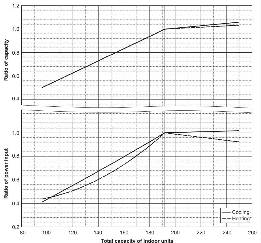
PQHY-P192T(S)LMU/Y(S)LMU-A
