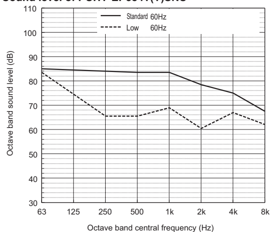
Sound level of PUHY-EP384T(Y)SNU
