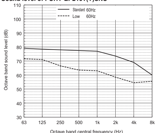
Sound level of PUHY-EP216T(Y)SNU
