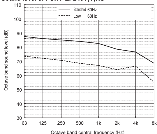
Sound level of PUHY-EP240T(Y)NU
