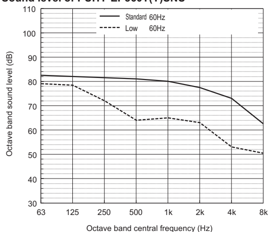
Sound level of PUHY-EP360T(Y)SNU
