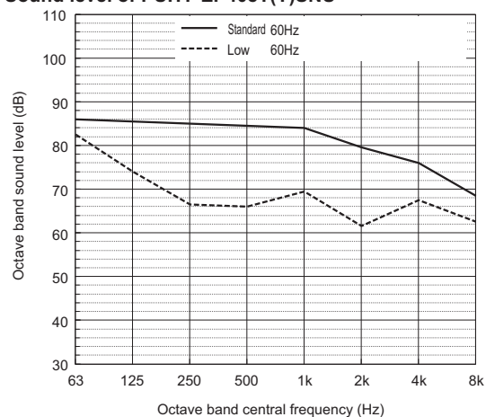
Sound level of PUHY-EP408T(Y)SNU
