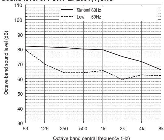
Sound level of PUHY-EP288T(Y)SNU
