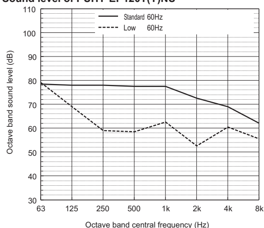
Sound level of PUHY-EP120T(Y)NU
