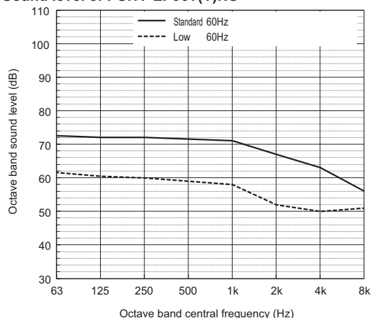
Sound level of PUHY-EP96T(Y)NU
