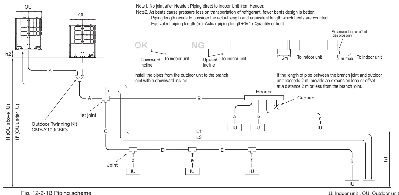
Fig. 12-2-1B Piping scheme
