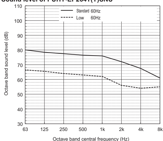
Sound level of PUHY-EP264T(Y)SNU
