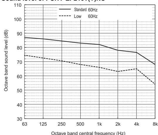
Sound level of PUHY-EP216T(Y)NU
