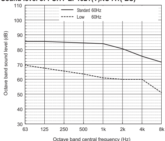
Sound level of PUHY-EP192T(Y)NU-A1(-BS)
