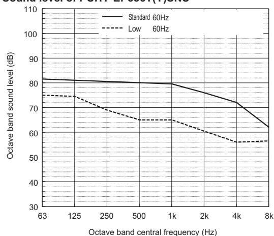
Sound level of PUHY-EP336T(Y)SNU
