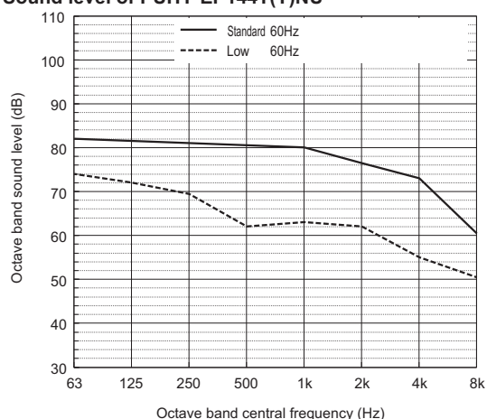
Sound level of PUHY-EP144T(Y)NU
