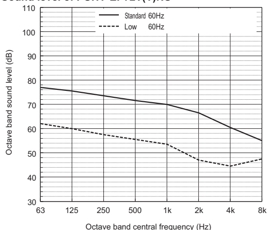
Sound level of PUHY-EP72T(Y)NU
