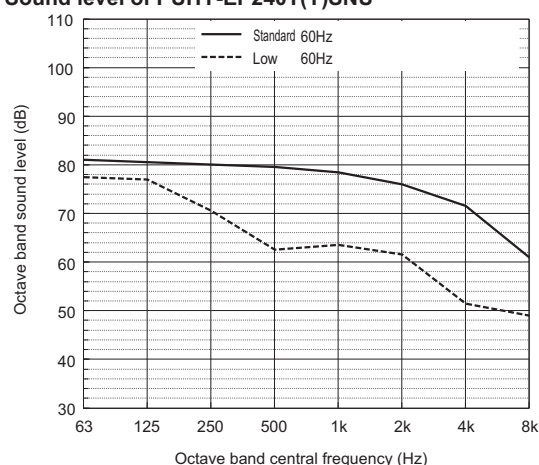
Sound level of PUHY-EP240T(Y)SNU
