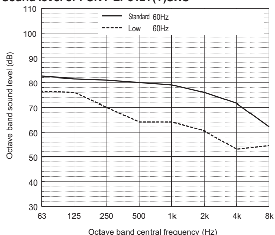
Sound level of PUHY-EP312T(Y)SNU
