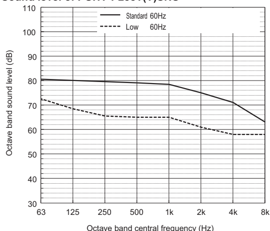
Sound level of PUHY-P288T(Y)SNU
