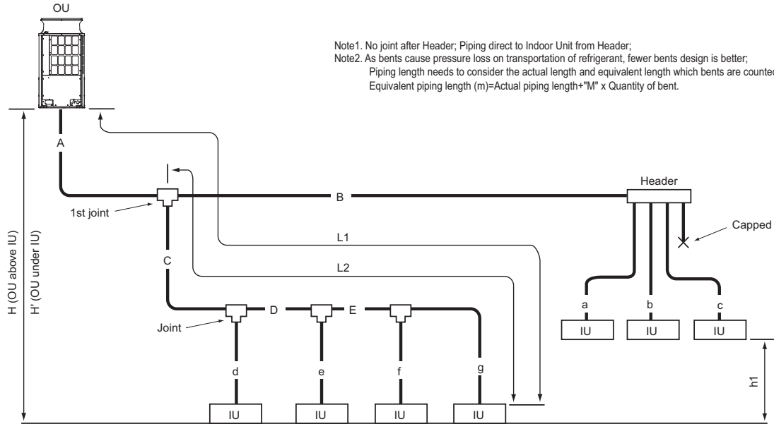
Fig. 12-2-1A Piping scheme
