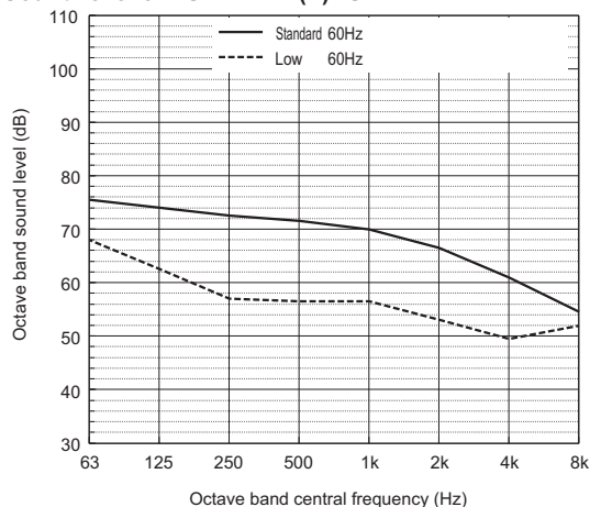
Sound level of PUHY-P72T(Y)NU
