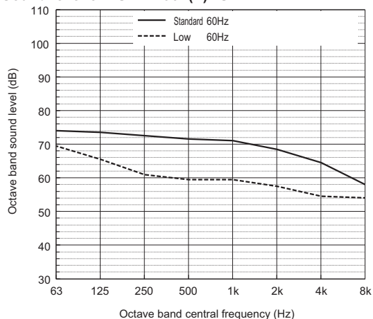
Sound level of PUHY-P96T(Y)NU
