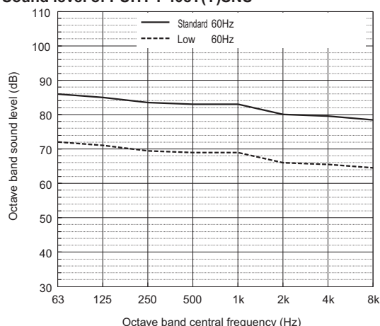
Sound level of PUHY-P408T(Y)SNU
