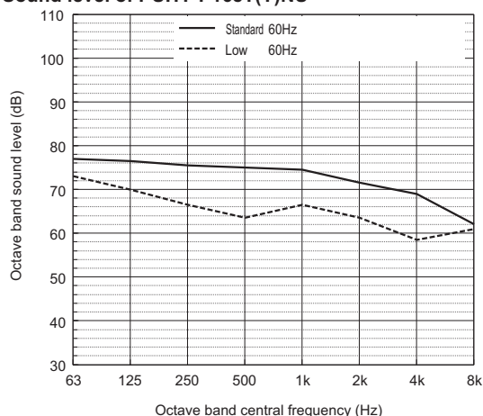
Sound level of PUHY-P168T(Y)NU
