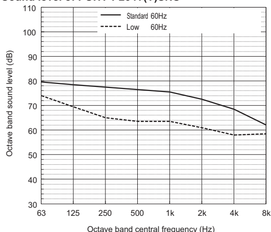
Sound level of PUHY-P264T(Y)SNU
