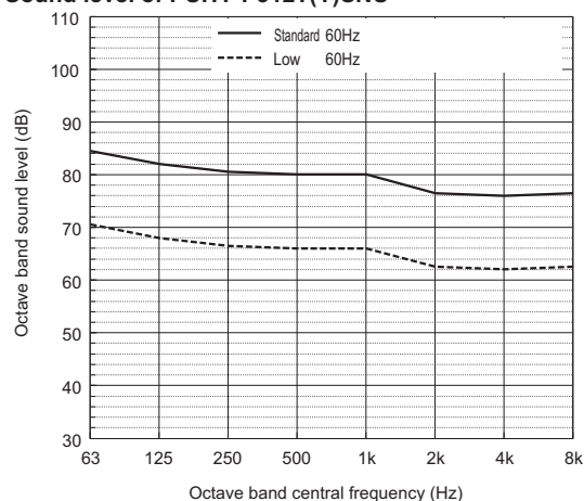
Sound level of PUHY-P312T(Y)SNU
