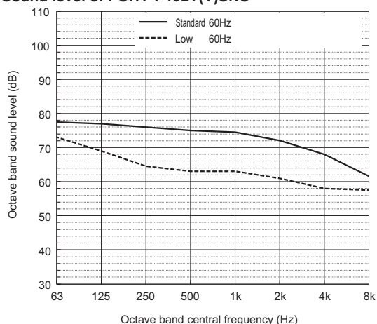
Sound level of PUHY-P192T(Y)SNU
