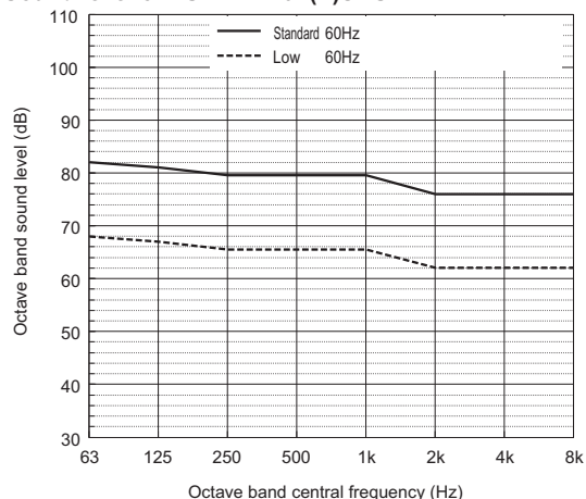
Sound level of PUHY-P240T(Y)SNU
