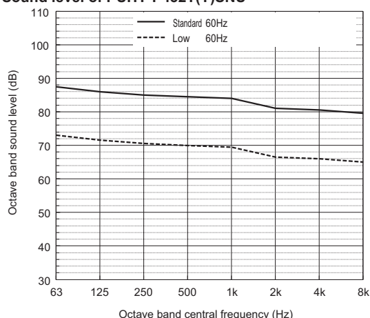
Sound level of PUHY-P432T(Y)SNU
