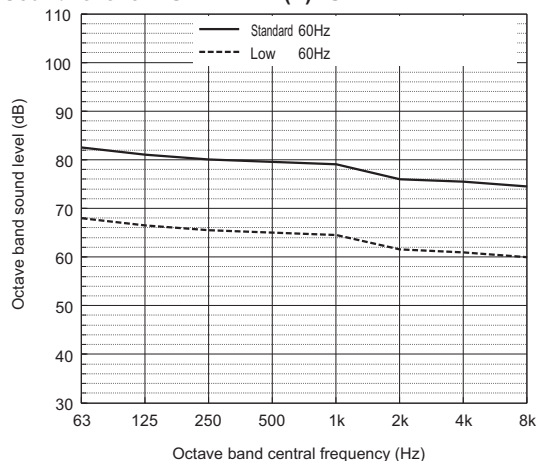
Sound level of PUHY-P144T(Y)NU
