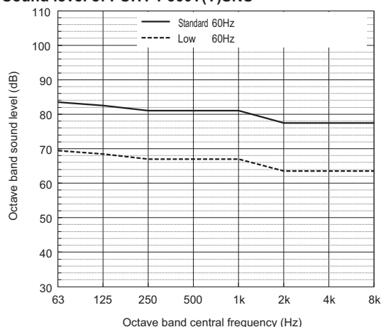
Sound level of PUHY-P360T(Y)SNU
