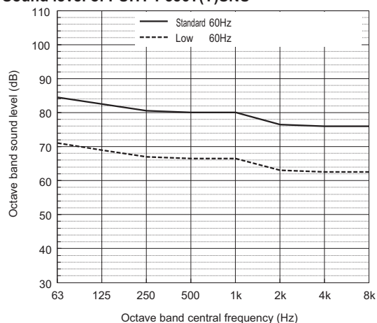
Sound level of PUHY-P336T(Y)SNU
