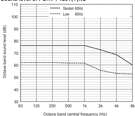
Sound level of PUHY-P120T(Y)NU
