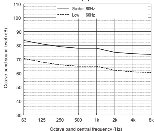
Sound level of PUHY-P216T(Y)SNU
