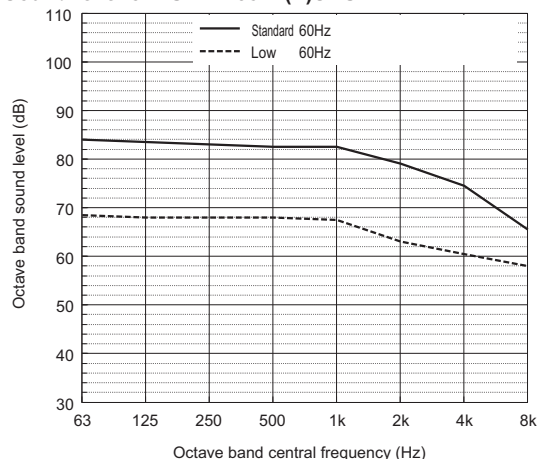
Sound level of PUHY-P384T(Y)SNU
