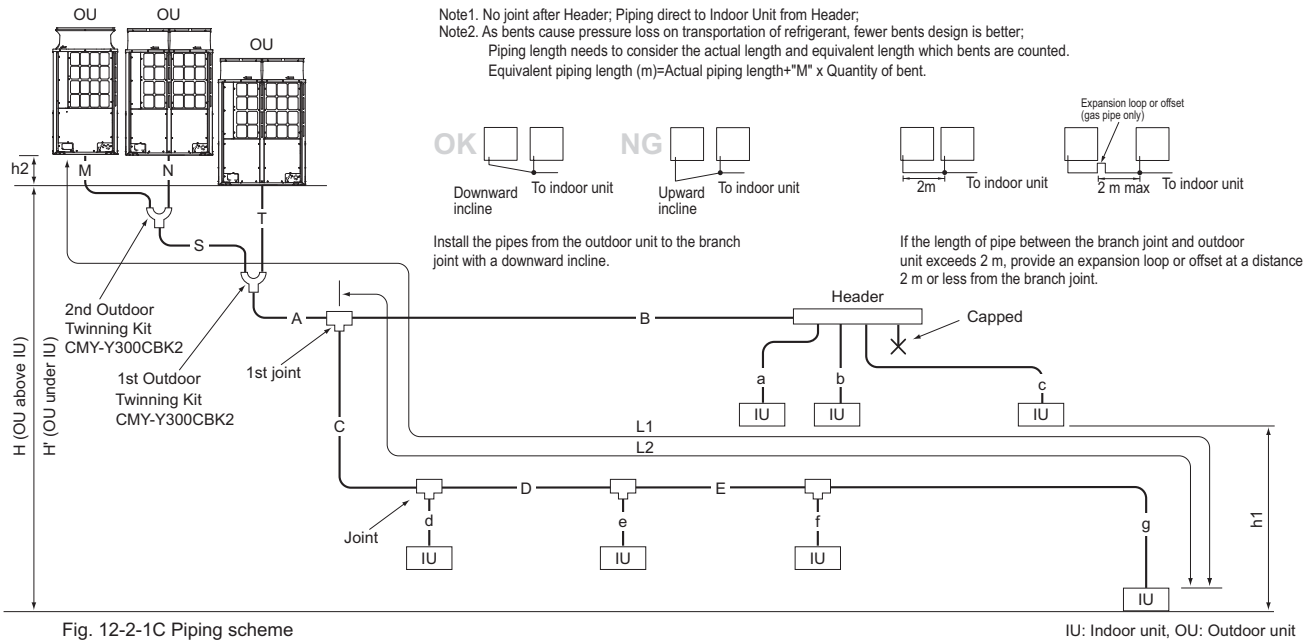
Fig. 12-2-1C Piping scheme
