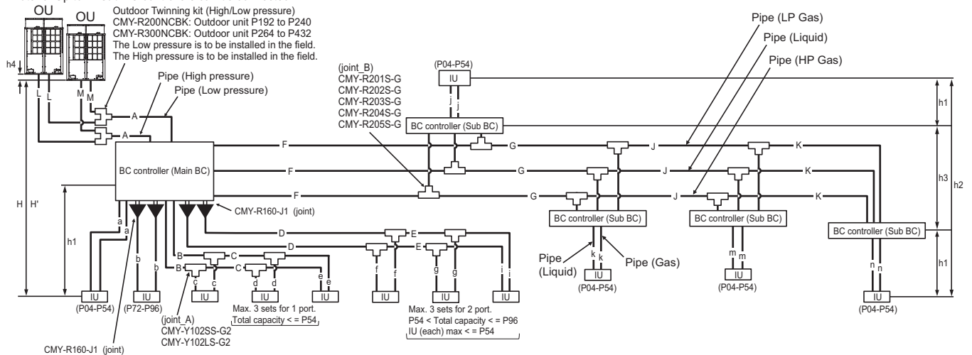
Fig. 12-2-3A Piping scheme
