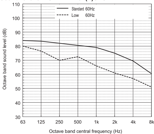
Sound level of PURY-EP240T(Y)SNU
