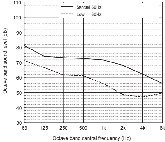
Sound level of PURY-EP72T(Y)NU
