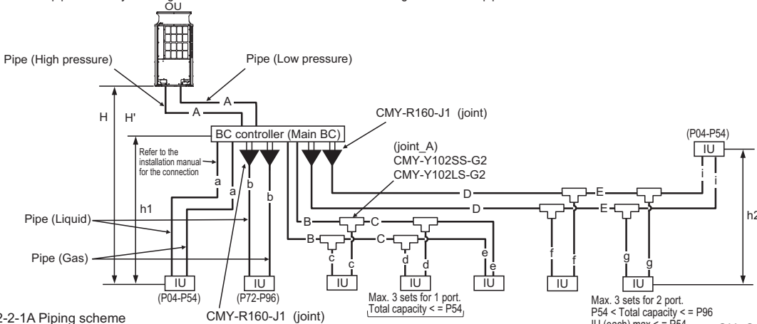
Fig. 12-2-1A Piping scheme
