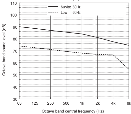
Sound level of PURY-EP432T(Y)SNU
