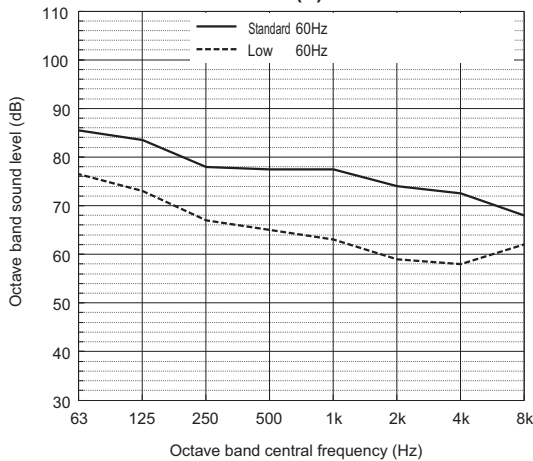
Sound level of PURY-EP192T(Y)SNU
