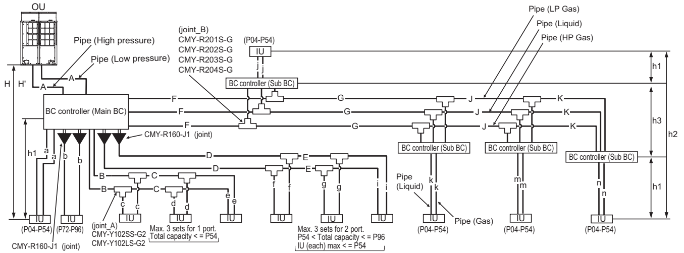
Fig. 12-2-2A Piping scheme
