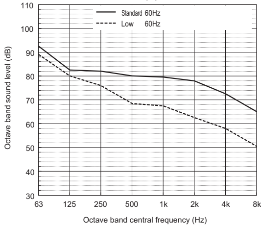
Sound level of PURY-EP336T(Y)SNU
