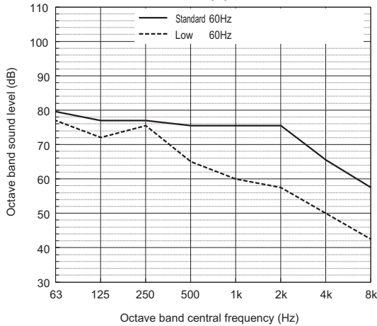
Sound level of PURY-EP120T(Y)NU
