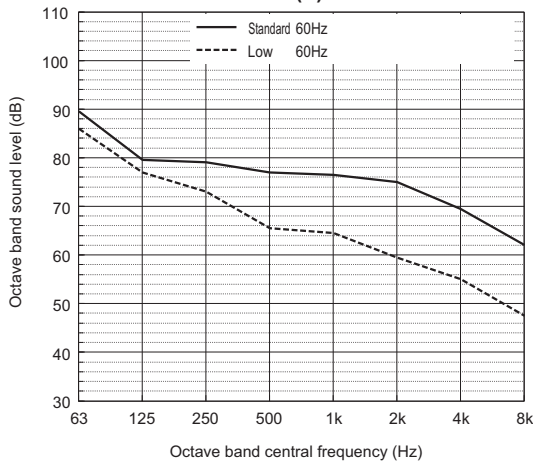
Sound level of PURY-EP168T(Y)NU
