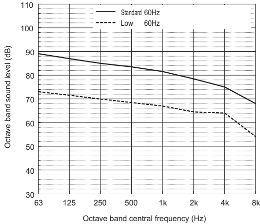
Sound level of PURY-EP216T(Y)NU
