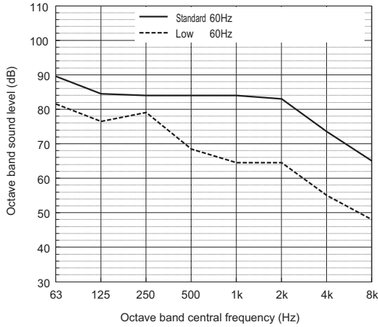
Sound level of PURY-EP288T(Y)SNU
