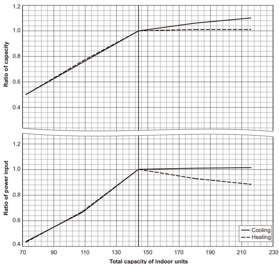
PURY-P144TNU/YNU-A
