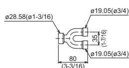
High-pressure twinning pipe
