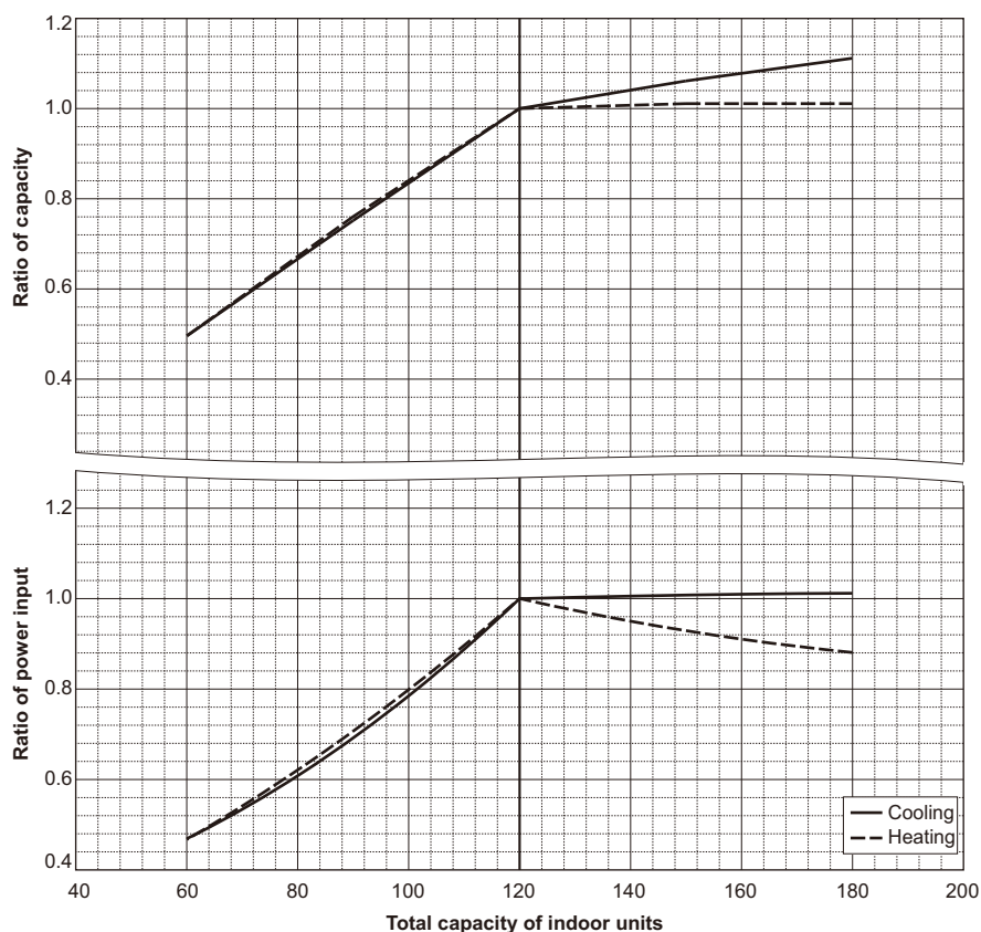
PURY-P144TNU/YNU-A
