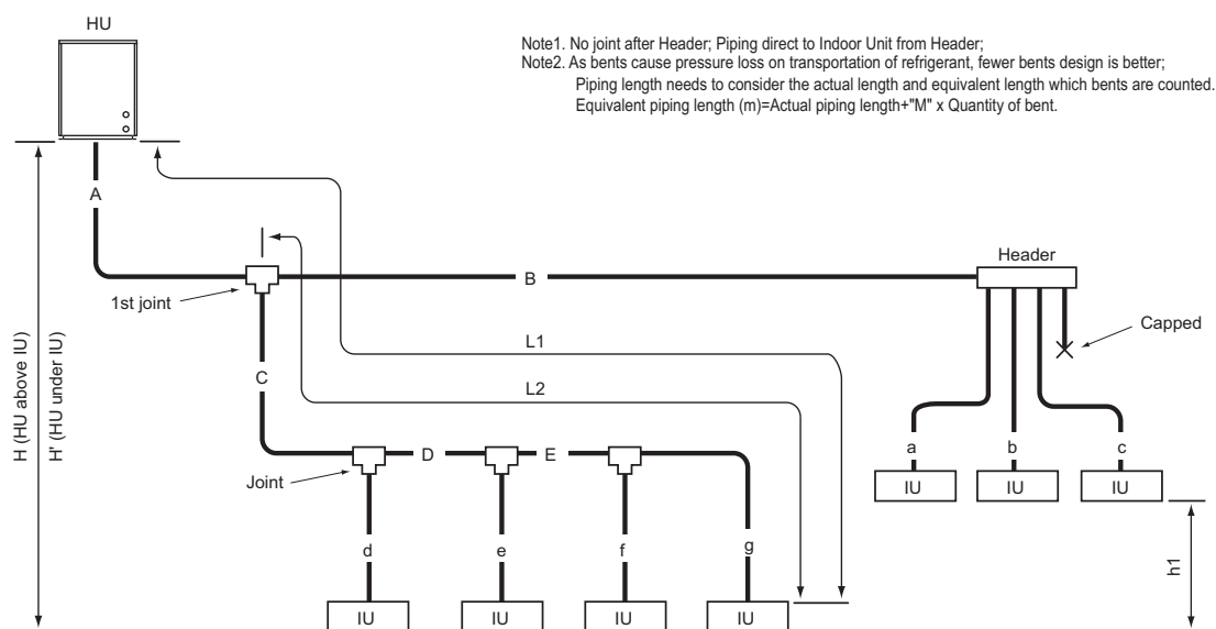
Fig. 3-2-1A Piping scheme
