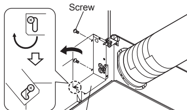
Control box cover Model LGH-F1200 RX5-E1
