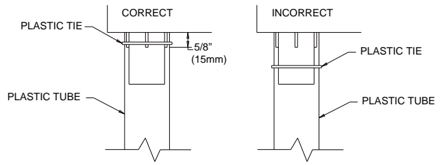
DETAIL A
