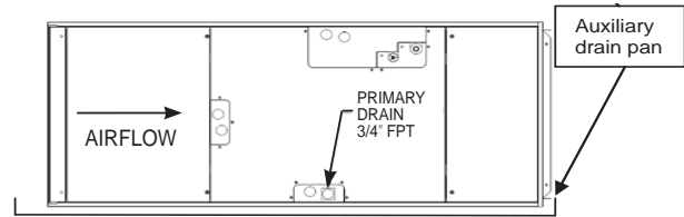
Horizontal Right Fan assembly rotation not required
