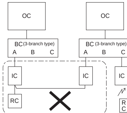
3-2. Group operation between different refrigerant systems
