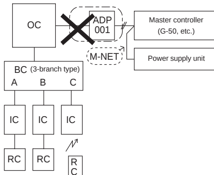
3-3. Connection of M-NET adapter to outdoor unit
