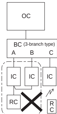
3-1. Group operation by single remote controller
