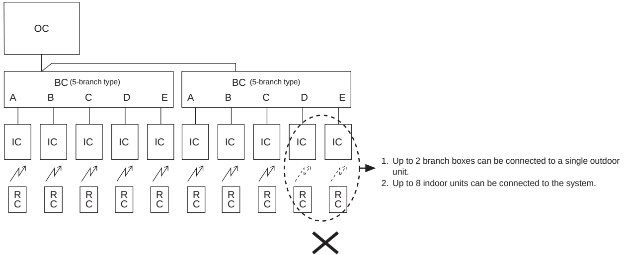
2-4. 2 branch boxes (5-branch type, maximum 8 indoor units)
