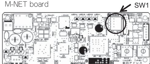
M-NET board
