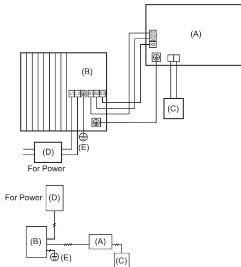
Indoor unit power supplied from outdoor unit
