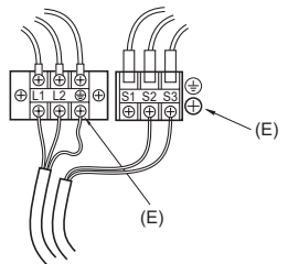
Separate indoor unit /outdoor unit power supplies
