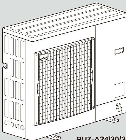
PUZ-A24/30/36NHA6 PUY-A24/30/36NHA6
