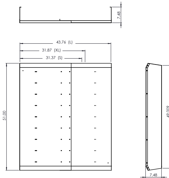
CM-WD-RE-TKMU (Universal fitting S, L, XL)
