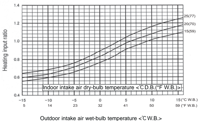
Fig. 2-2 Heating input
