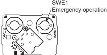
CN303 Indoor controller board (I.B.) Connected to CNRU
